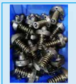
No.543(5) :CP4 Plunger
