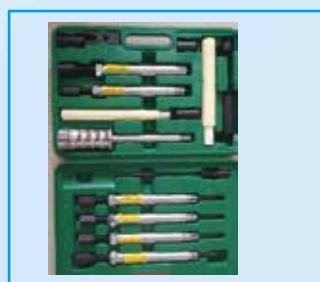
No,052 Tools for CR Injector Bushings
