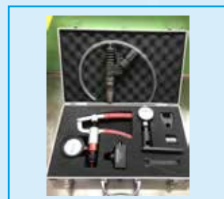
No.128(3) ISM CUMMINS M11,N14 Injector Valve Stroke Measuring Tools
