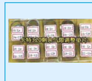
No. 121(2) CAT320 Residual Air Gap Adjustment Shims:10Kinds x 5pcs=50Pcs
