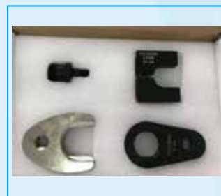
NO,105(8) EUI HYUNDAI 22880-84001 TOOLS
