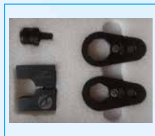
NO105(5) Dismounting Tools for Scania and Volvo
