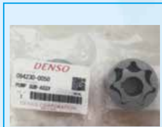
No,552(4) Feed Pump 094230-0040/ 094230-0050
