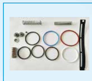
No. 125 Repair Kits For Cummins ISM Injector
