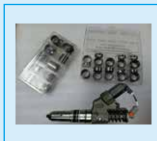
No.128(2) ISM CUMMINS M11,N14 Injector Valve Stroke Adjustment Gasket
