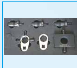
NO,105(1) Dismounting Tools For CATERPILLAR HEUI 3126/C7/C9
